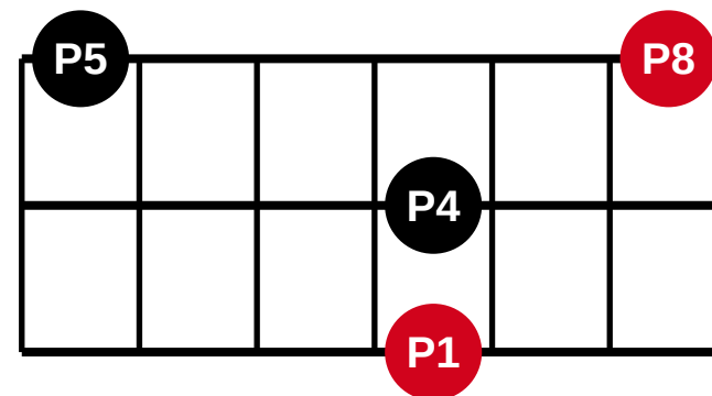
3 strings - 6 frets - fingering 3 of 3
