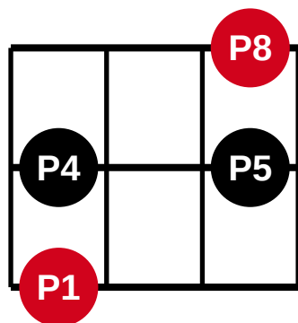
3 strings - 3 frets - fingering 1 of 3
