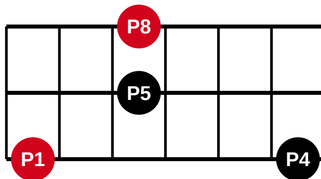
3 strings - 6 frets - fingering 2 of 3
